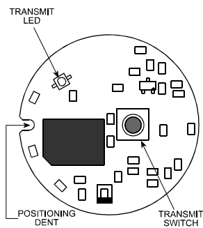
Figure 3. Transmitter Module - Top Side
