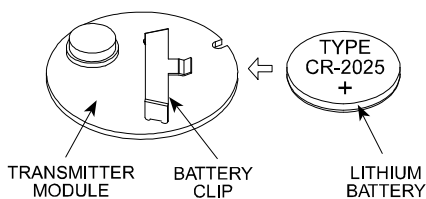
Figure 4. Battery Insertion
